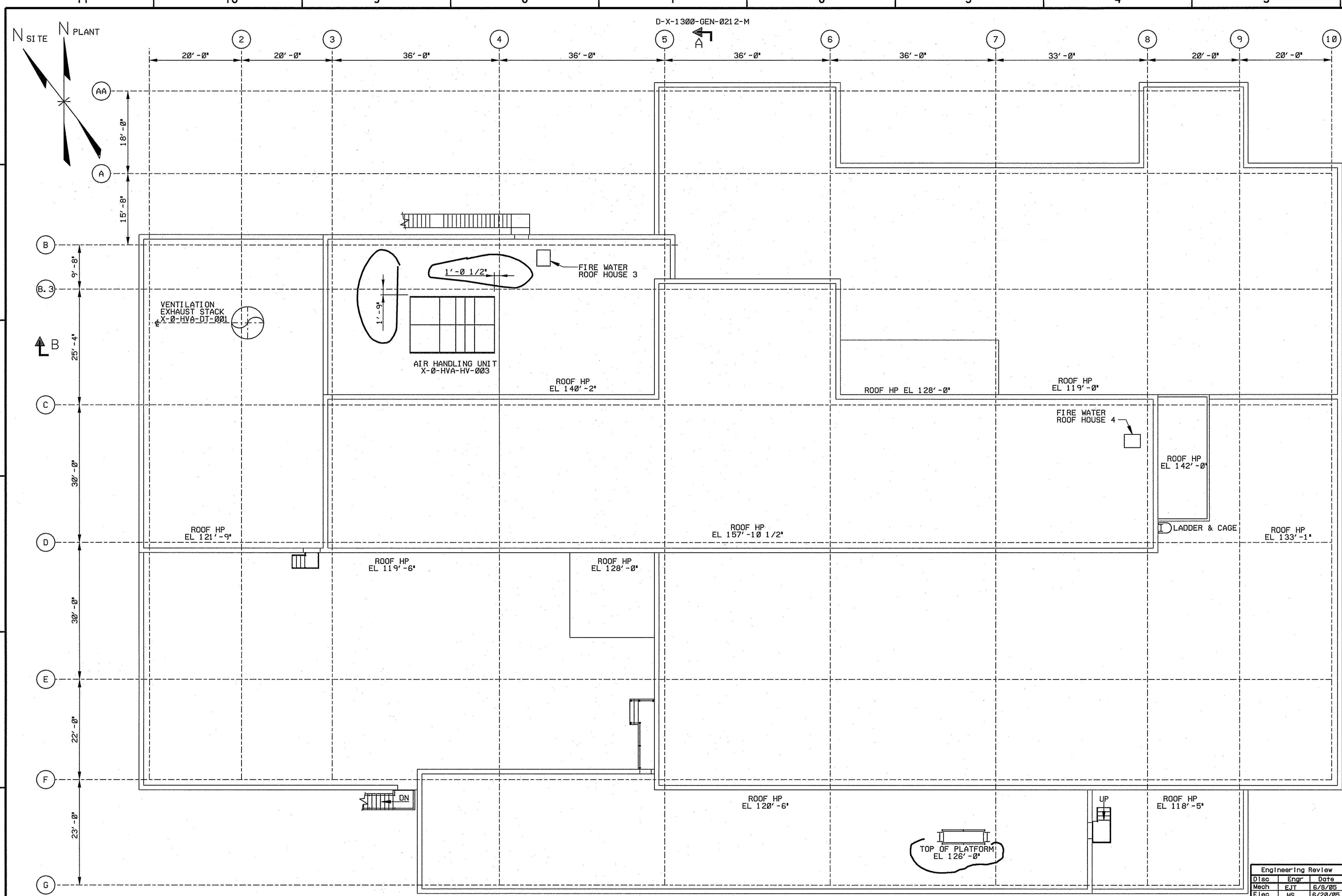
ROOF PLAN
